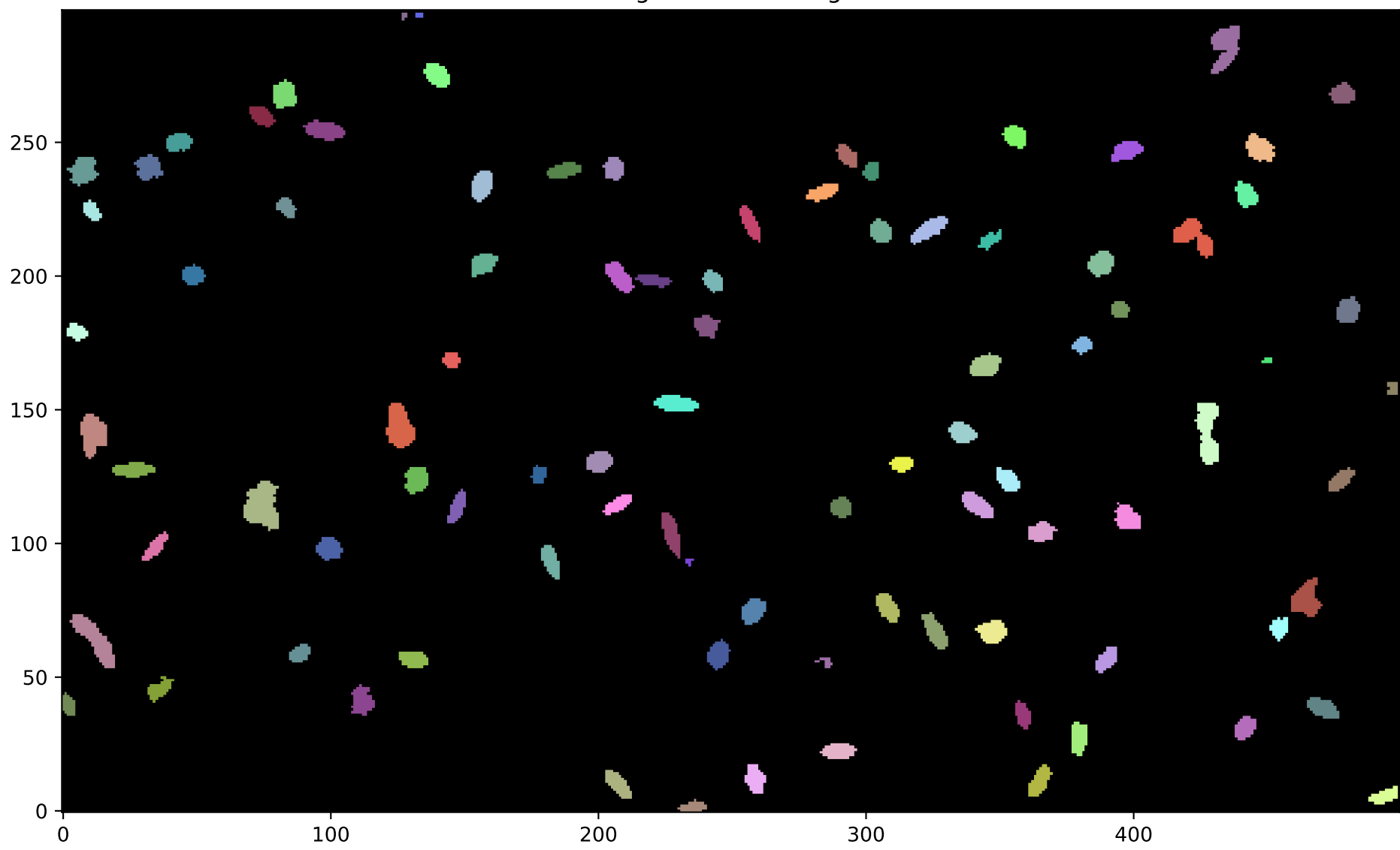
Segmentation Image
