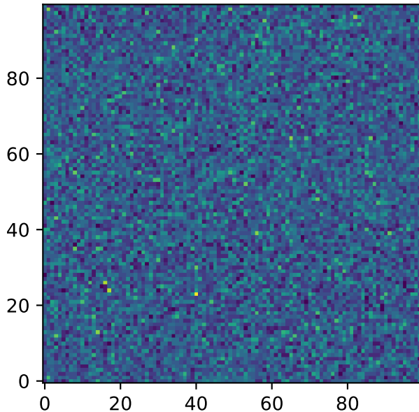
Poisson noise ( \mu = 5 )
