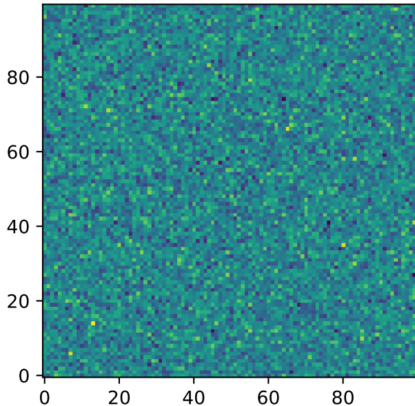
Gaussian noise ( \mu = 0, \sigma = 5. )
