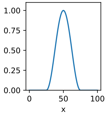
Cosine Bell
