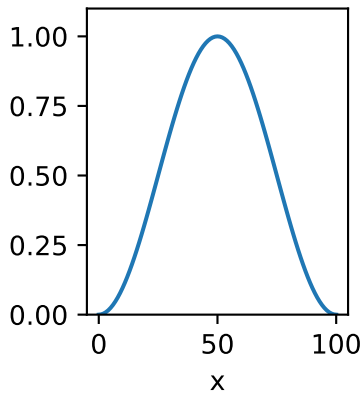
Hanning
