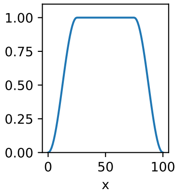
Tukey
