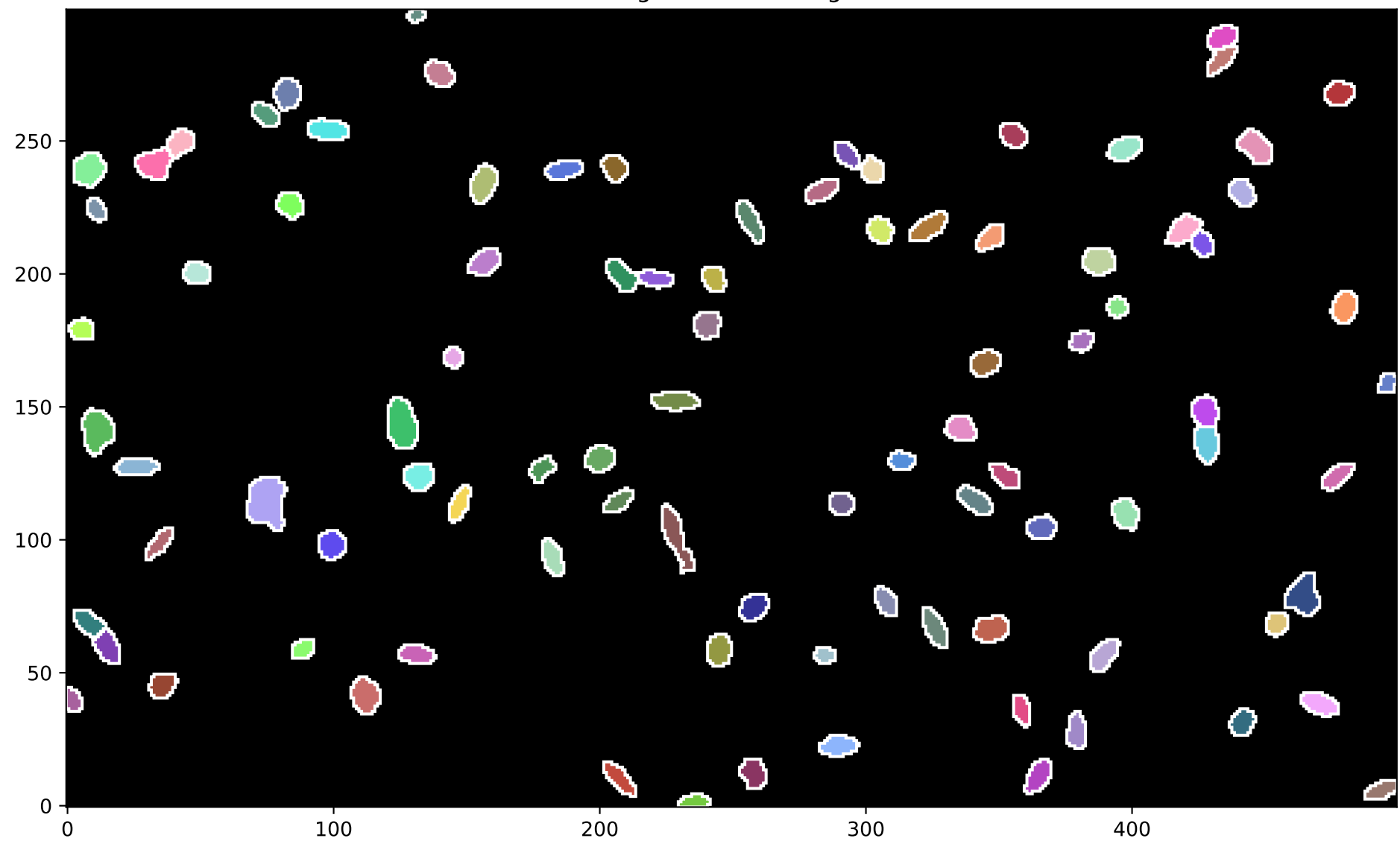
Background-subtracted Data
