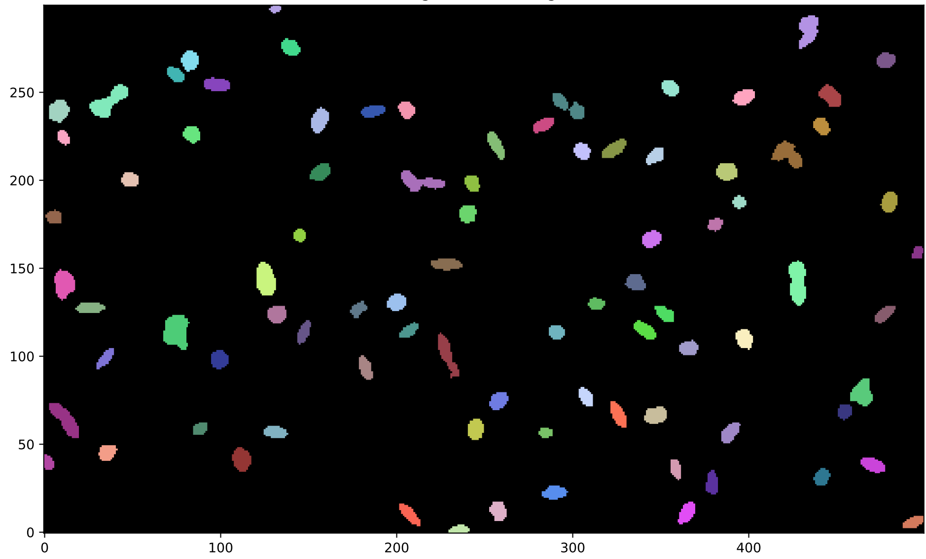
Segmentation Image
