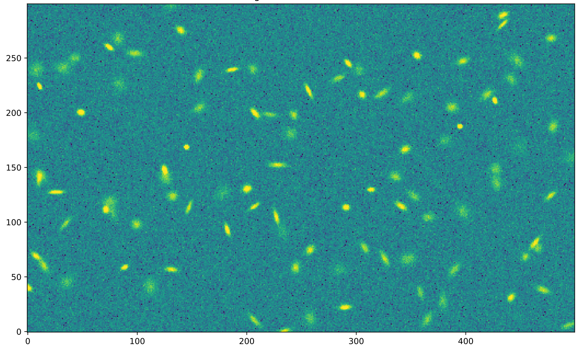
Segmentation Image
