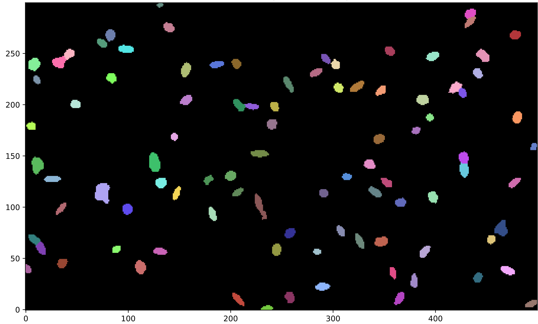
Deblended Segmentation Image
