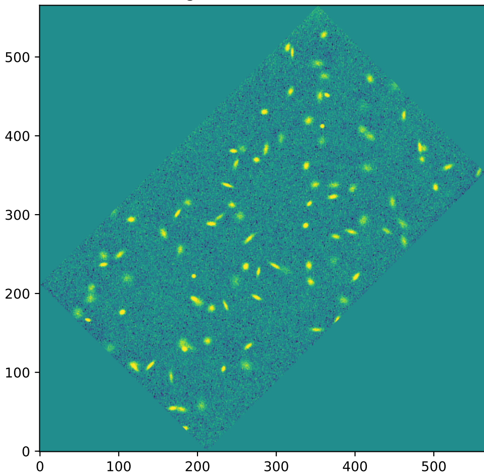
Background-subtracted Data
