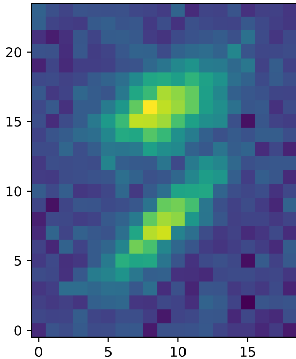
Background-subtracted Data
