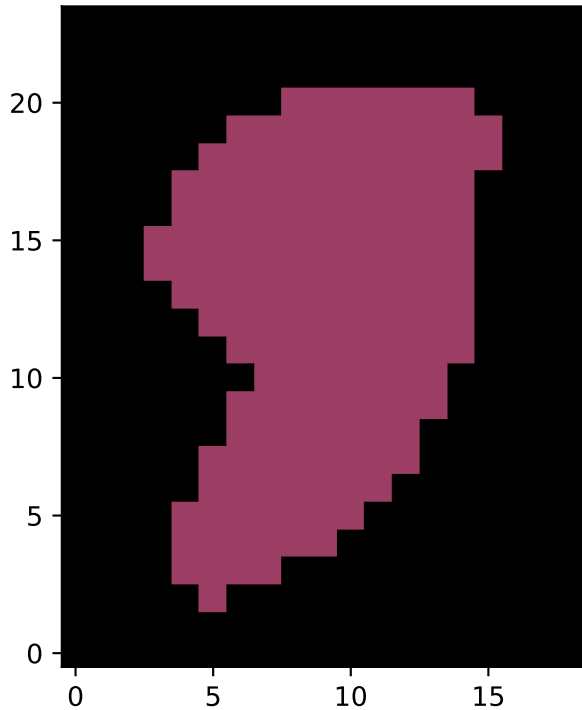
Original Segment
