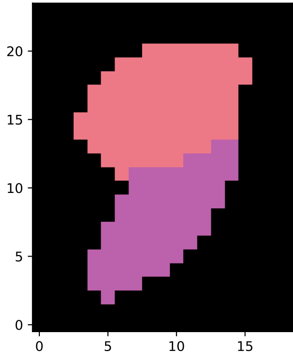
Deblended Segments
