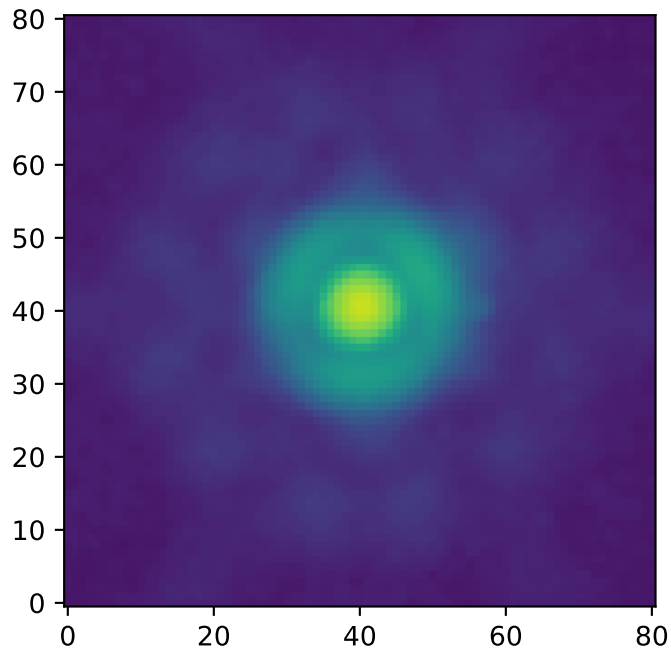
IRAC channel 4 PSF
