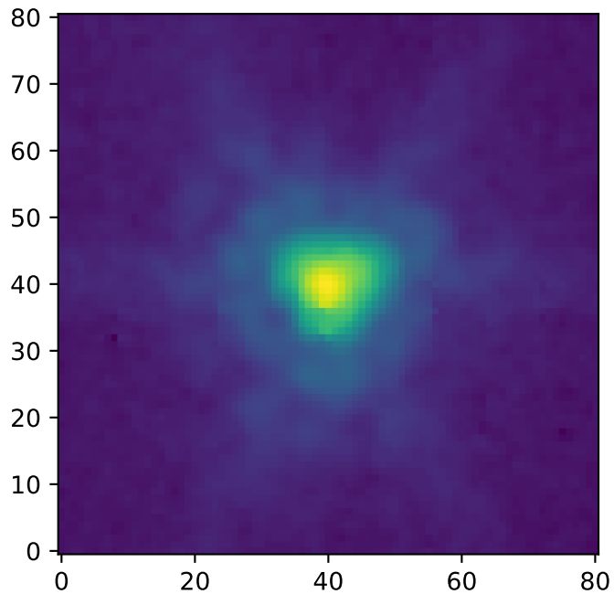
IRAC channel 1 PSF
